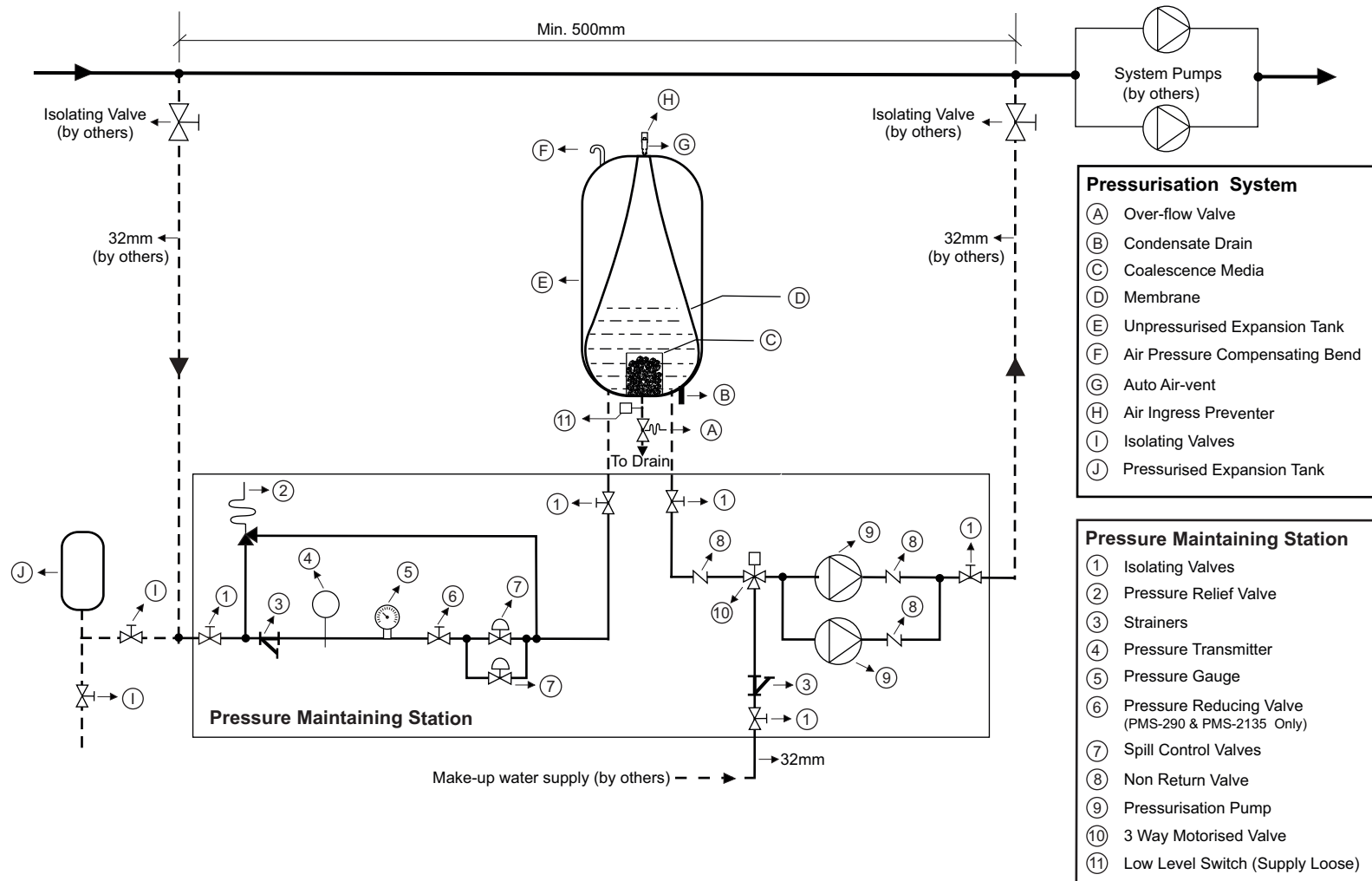
Typical Flow Diagram of Hydronic Pressurisation System
